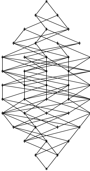
FIGURE 2. The poset \text{Br}(\iota(\theta)) when W = E_6 and \theta is the non-trivial automorphism.
